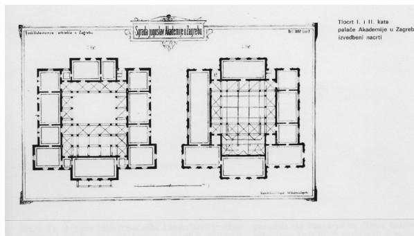
FRIEDRICH VON SCHMIDT, TLOCRT PALAČE AKADEMIJE / FRIEDRICH VON SCHMIDT, GROUND PLAN OF ACADEMY PALACE
